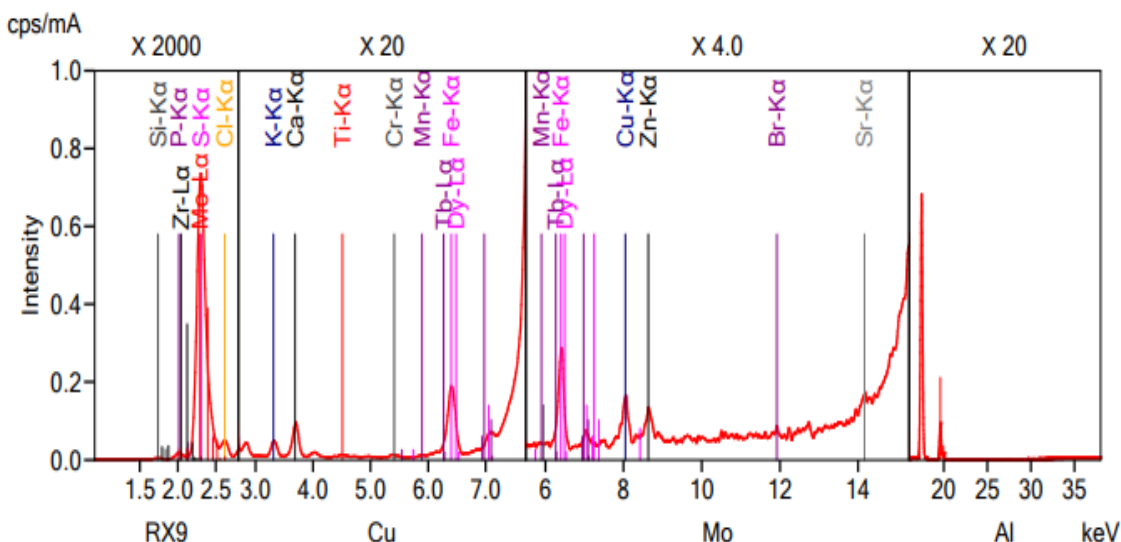
1-rasm. Mo (VI) bilan PPA polimer tashuvchiga immobillangan FF ning rentgen-fluorescent tahlili natijalari.
