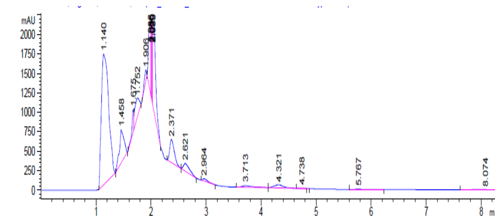
Fig.1. Chromatogram of the component composition of concentrated milk thistle seed extract.
