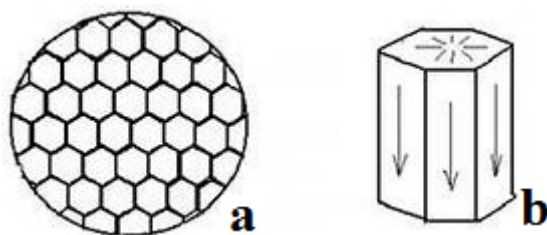
1 – rasm. Benar yacheykasi
