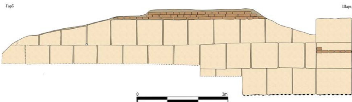
2-rasm. 1-xonaning shimoliy devoir qirqimi
